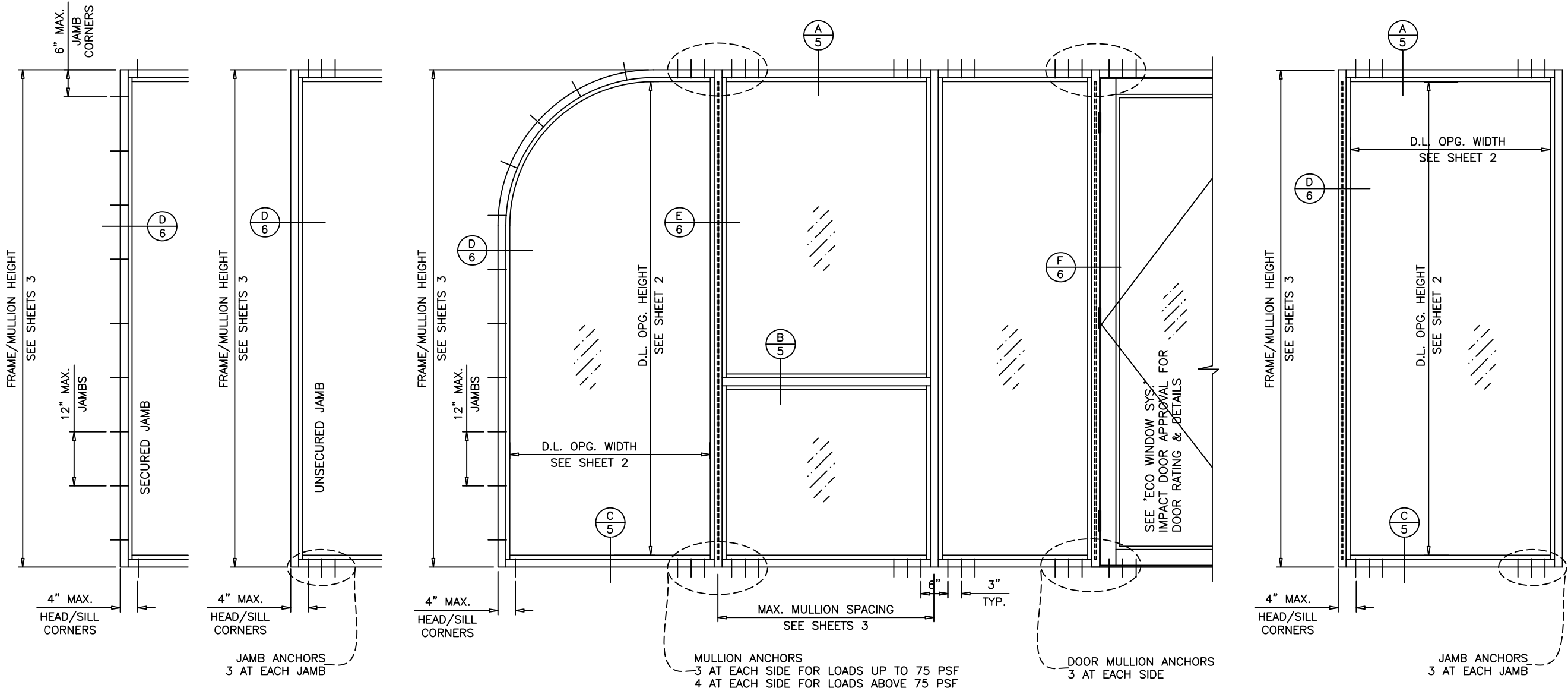
TYPICAL ELEVATION
